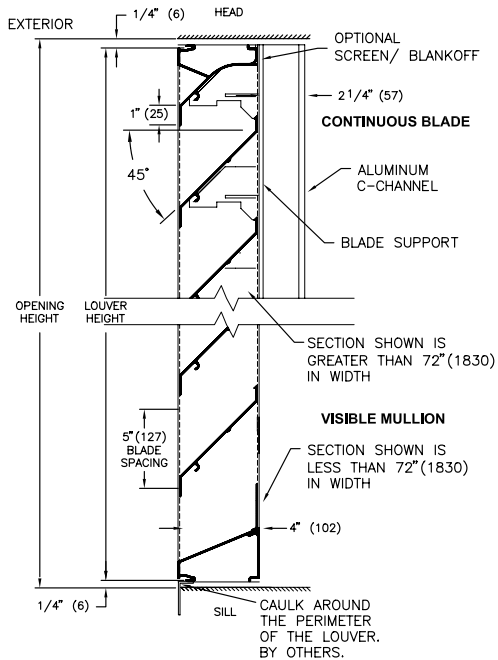
“A” Mounting
