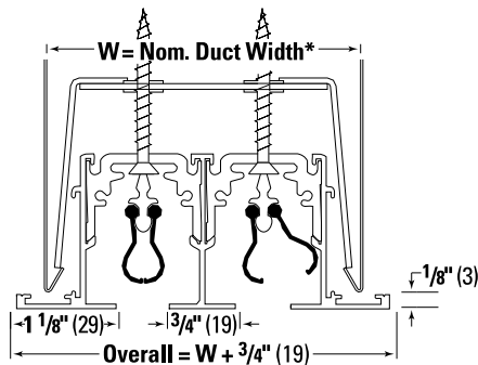
Surface Mount – Concealed Type 2 Flanged frame
