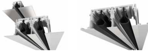
SDS, SIZES 0.75" (75) AND 1" (100)
