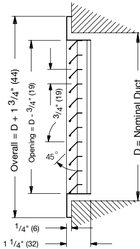
530 / F / L / A / B12 (White) 3/4" (19) Blade Spacing Fixed Louvers, No Damper
