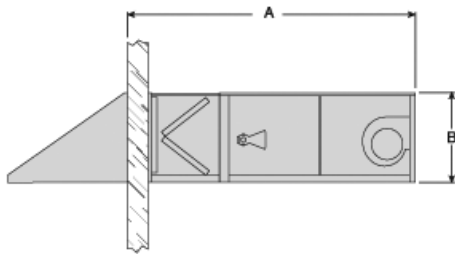
ERV - Energy Recovery Ventilations (Thru Wall Arrangement)
