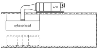
Outdoor / Horizontal Roof Mounted
