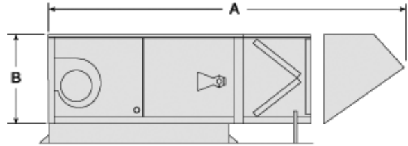
ERV Energy Recovery Ventilations (1. Downblast Discharge - Arrangement DB 2. Horizontal Discharge - Arrangement HZ)
